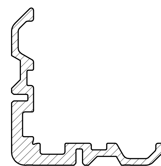
P010100 CORNER CLEAT 10mm
