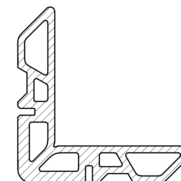
P010160 CORNER CLEAT 16mm
