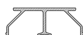
PP 2002 RAILS BASIN COVER
